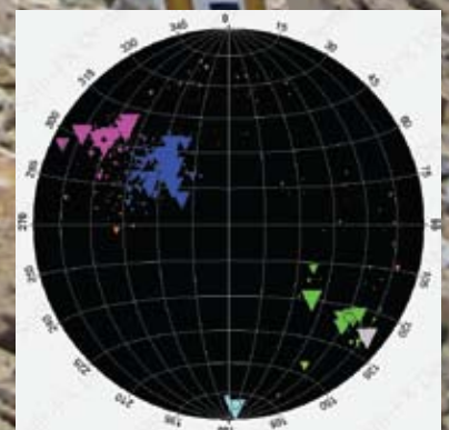
Stereonet
